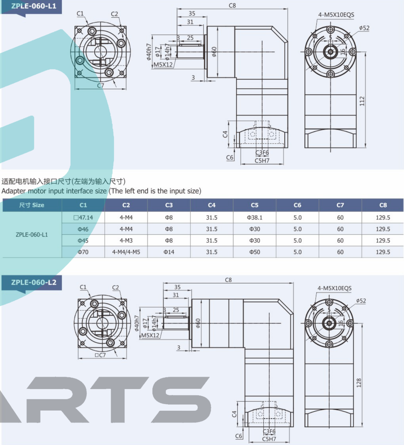
适配电机输入接口尺寸(左端为输入尺寸) Adapter motor input interface size (The left end is the input size)
