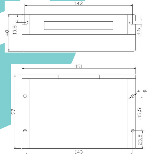
Figure 1: Mechanical specifications
