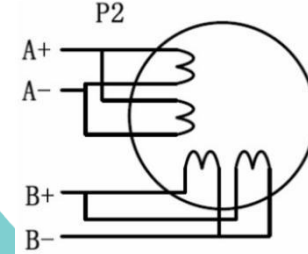
Figure 8: 8-lead motor parallel connections
