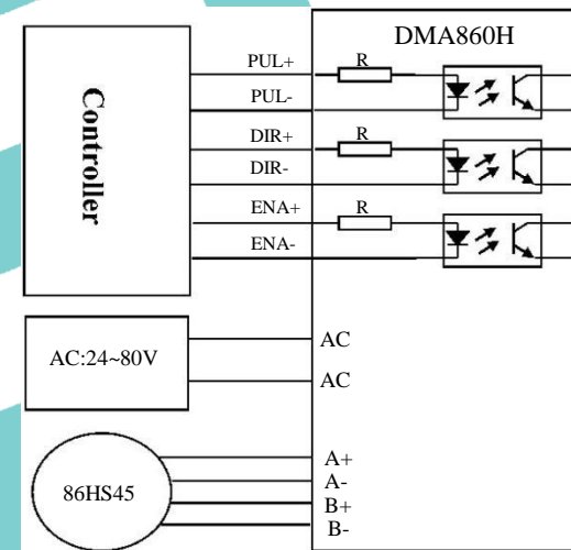
Figure 9 DMA860H Typical connection
