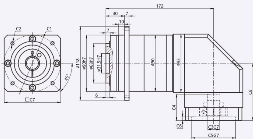
适配电机输入接口尺寸(左端为输入尺寸) Adapter motor input interface size (The left end is the input size)
