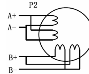
Figure 8: 8-lead motor parallel connections
