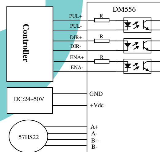
Figure 9 DM556 Typical connection
