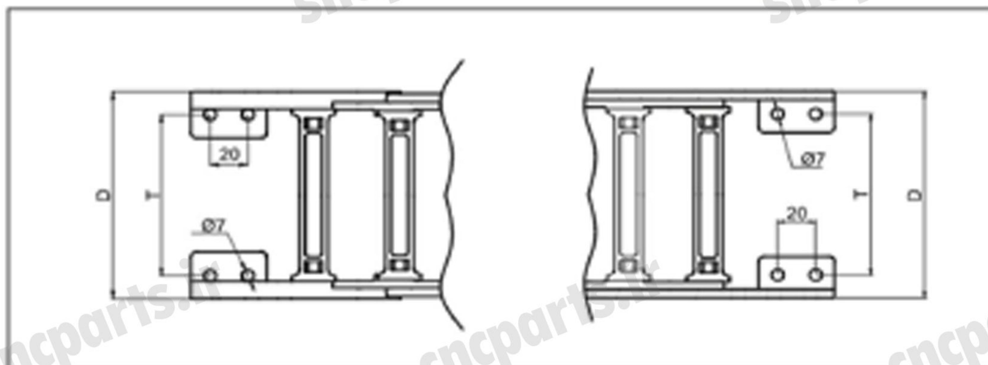
(Plastic End Brackets Connection)
